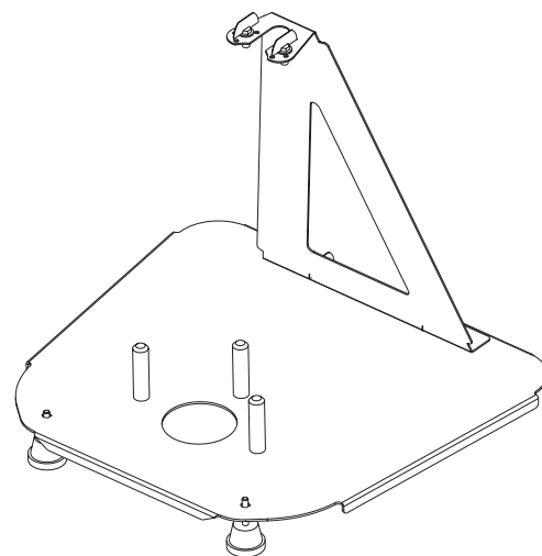
Art. CS2/CS4 BASE (optional): for vertical installation
